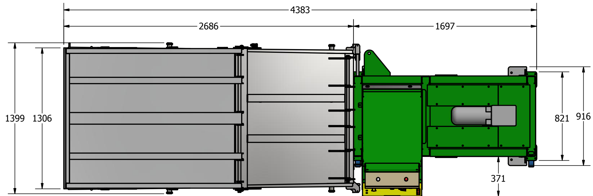
PLAN VIEW
